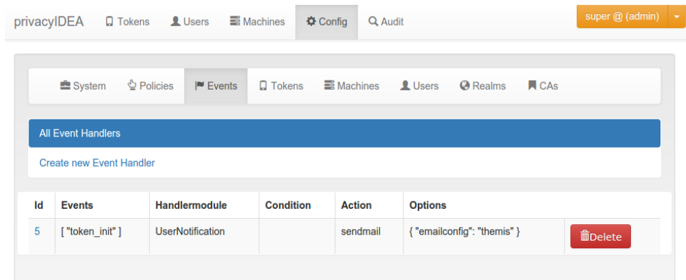
Fig. 70: An action is bound to the event token_init.
