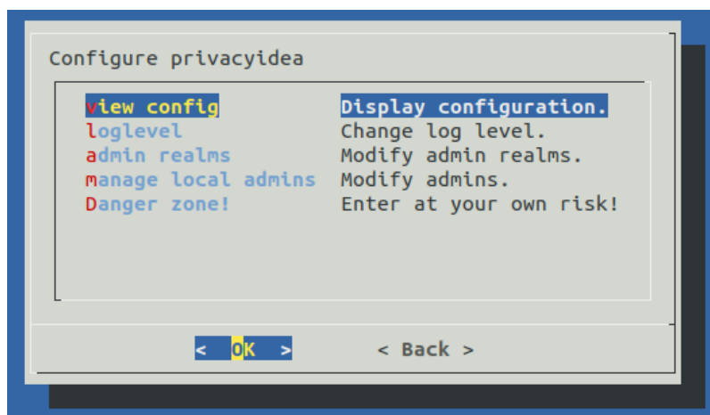
Fig. 35: Configure privacyidea
