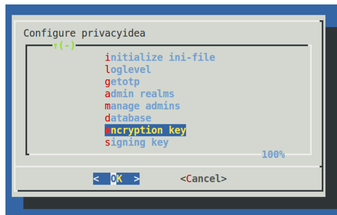
Fig. 31: Configure privacyidea
