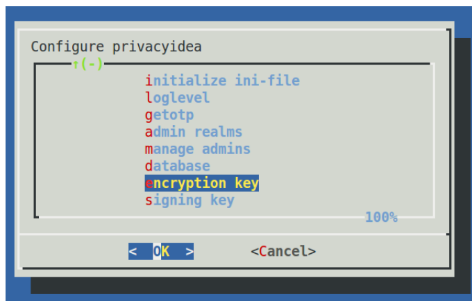
Fig. 40: Configure privacyidea
