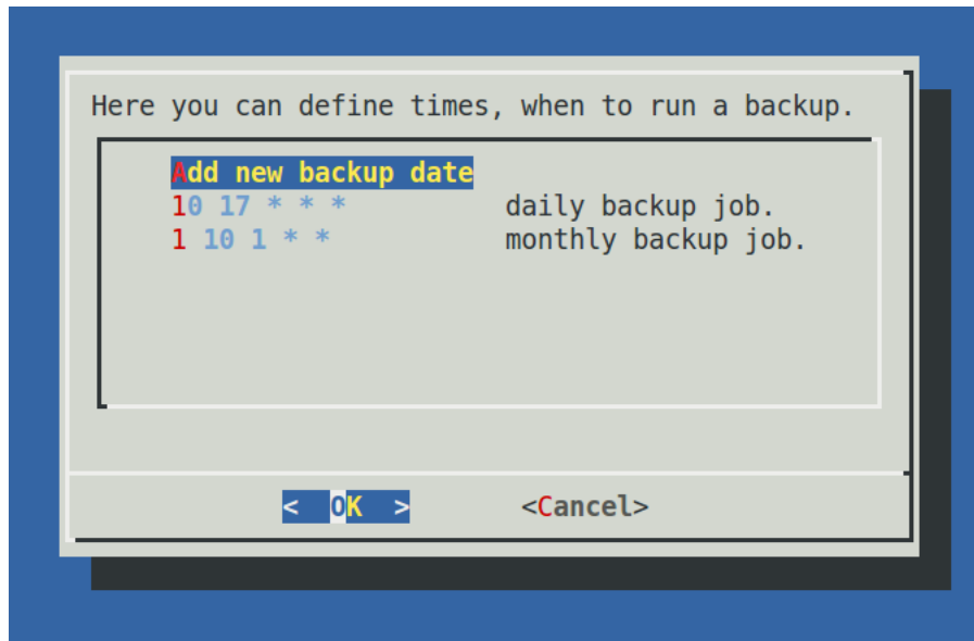
Fig. 43: Scheduled backup
