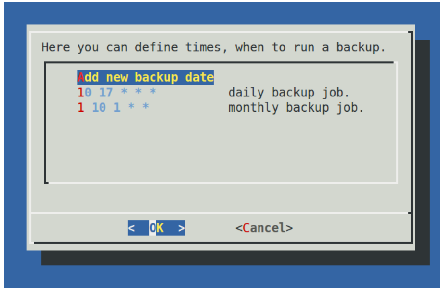
Fig. 43: Scheduled backup
