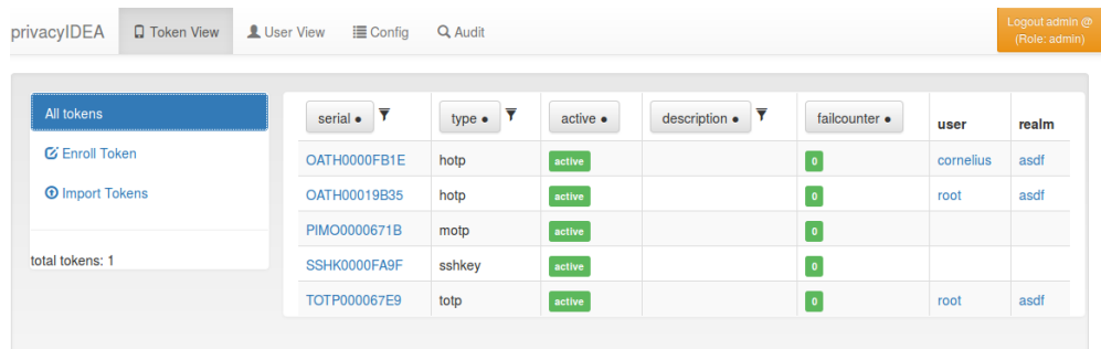
Fig. 46: Token View
