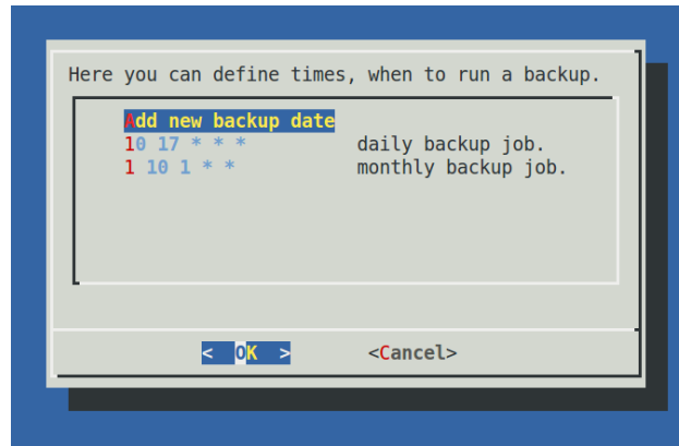
Fig. 1.39: Scheduled backup
