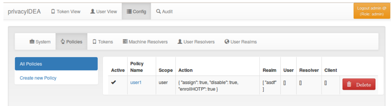
Fig. 1.50: Policy Definition
