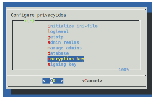
Fig. 1.36: Configure privacyidea
