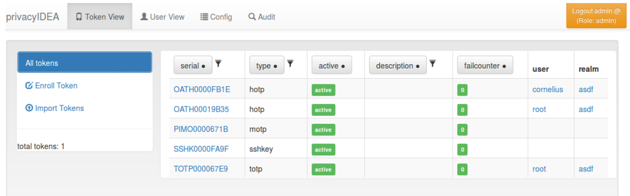
Fig. 1.41: Token View
