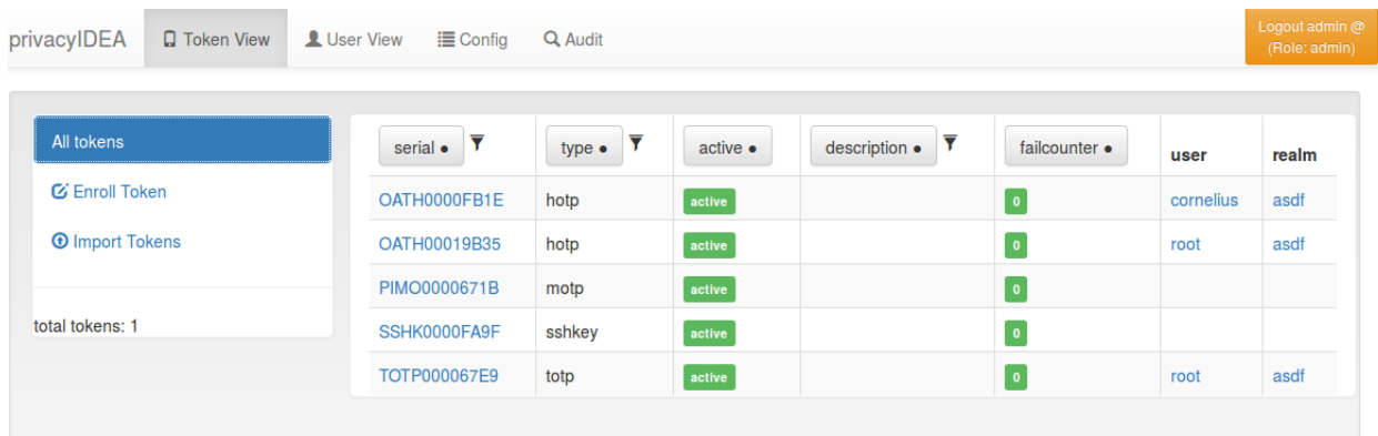
Fig. 1.46: Token View
