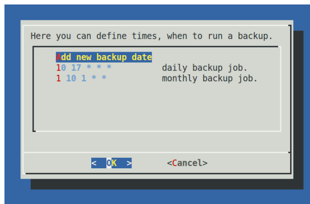
Fig. 1.43: Scheduled backup
