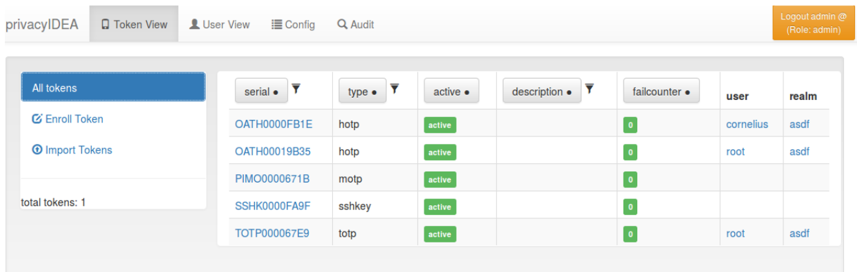
Fig. 1.46: Token View
